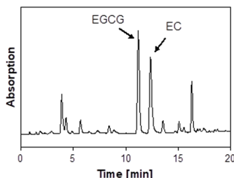
Fig. 1: Example chromatogram of green tea.
